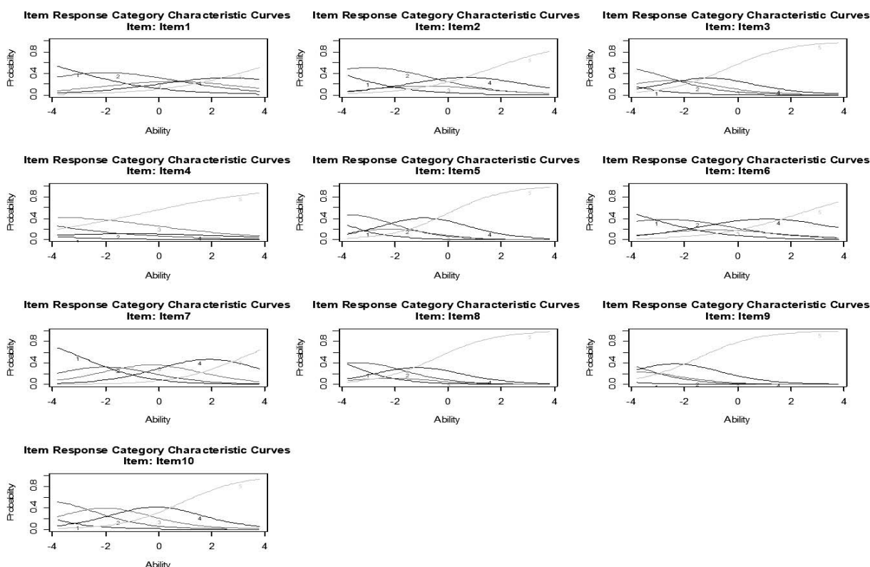
Figure 2 - Item characteristic curves for Form 2 administered in May 2018.
